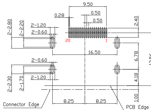
RECOMMENDED PCB LAYOUT (THICKNESS=1.6)
