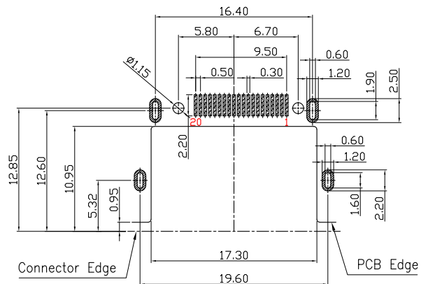
RECOMMENDED PCB LAYOUT (THICKNESS=1.20)
