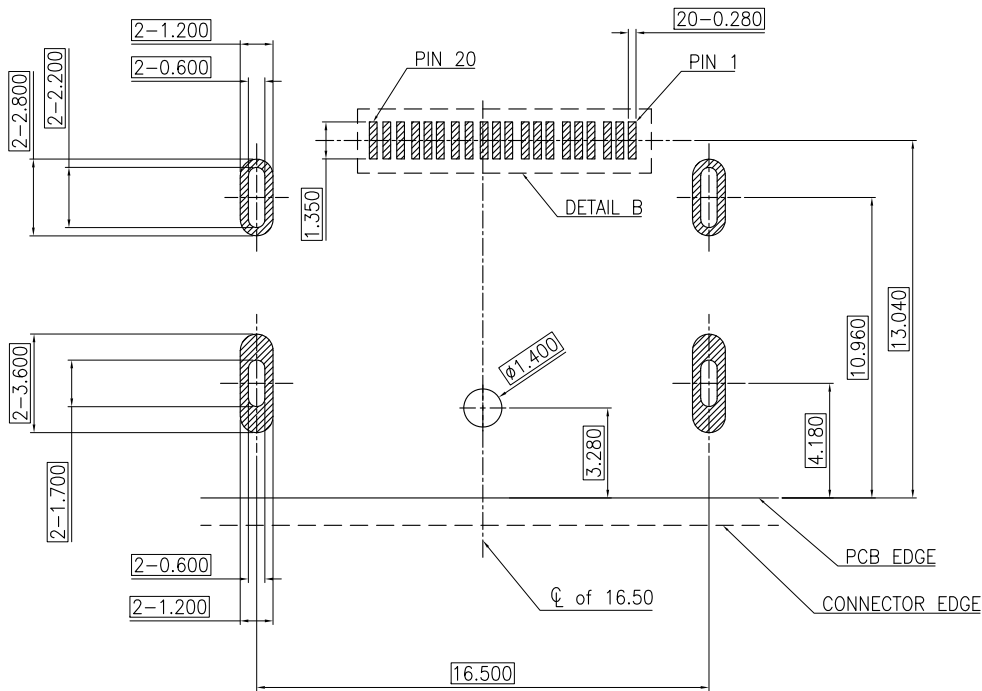
RECOMMENDED PCB LAYOUT ENHANCED FSDP TYPE 2 FOOTPRINT SCALE 2:1
