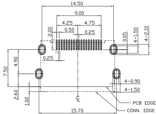
RECOMMENDED P.C.B LAYOUT (TOP VIEW) PCB THICKNESS:1.60MM
