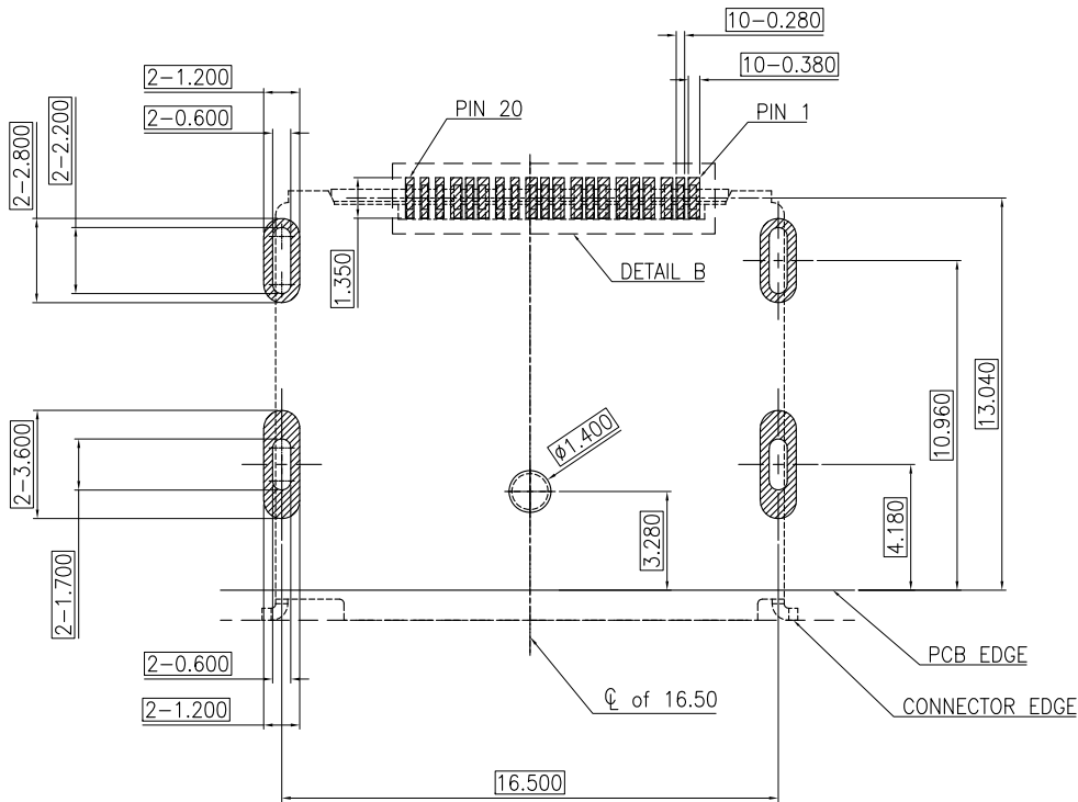
RECOMMENDED PCB LAYOUT ENHANCED FSDP TYPE 2 FOOTPRINT SCALE 2:1
