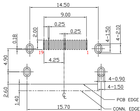
RECOMMENDED P.C.B LAYOUT (TOP VIEW) PCB THICKNESS:1.60MM
