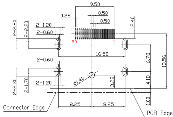
RECOMMENDED PCB LAYOUT (THICKNESS=1.6)
