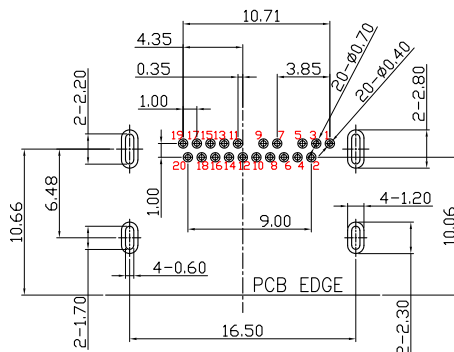
RECOMMENDED PCB LAYOUT (THICKNESS=1.6)
