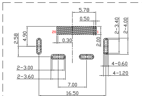
RECOMMENDED DP PCB LAYOUT (COMPONENT SIDE) THICKNESS=1.20±0.05 (TOP VIEW) DEFAULT TOL ±0.05
