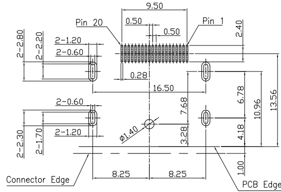
RECOMMENDED PCB LAYOUT (THICKNESS=1.6)
